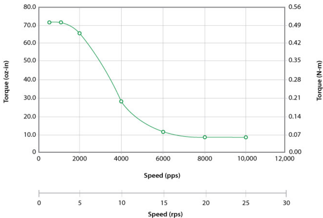
G4518L-02 24VDC, 1.35 Amps/Phase, Bipolar, 1/2 Stepping
